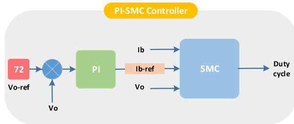
Fig. 3. PI-SMC voltage controller
