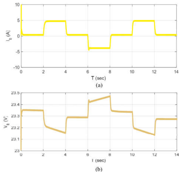
Fig. 8. BESS Performance. (a) Battery current, (b) Battery voltage
