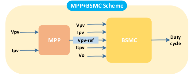
Fig. 2. MPPT controller
