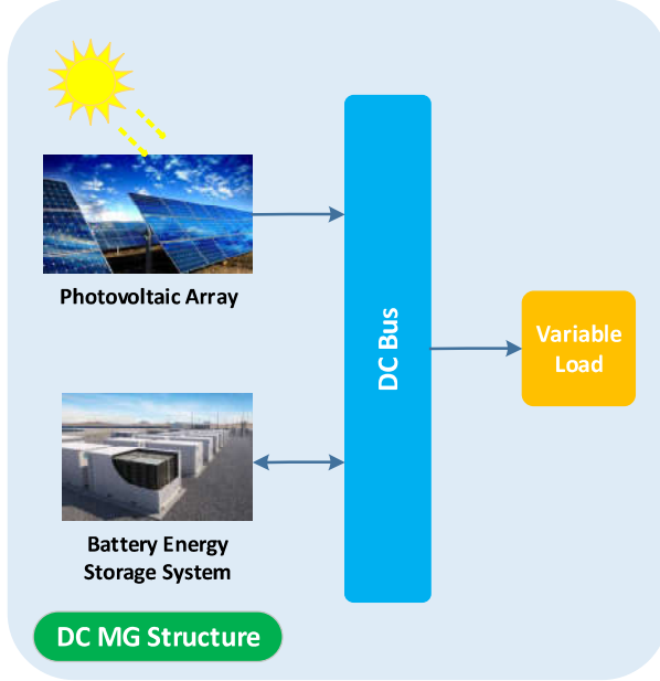
Fig. 1. The proposed islanded DC microgrid
