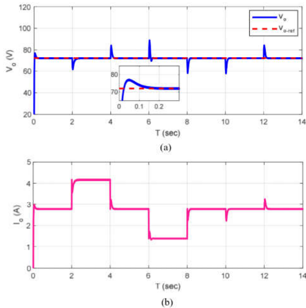
Fig. 6. DC MG load results. (a) DC link voltage, (b) Output load voltage
