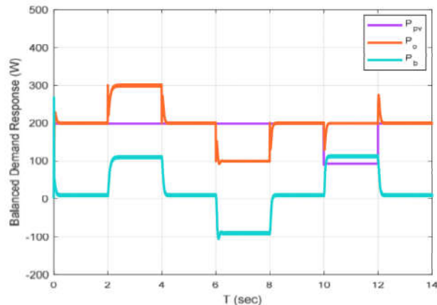
Fig. 7. Balanced Demand Response
