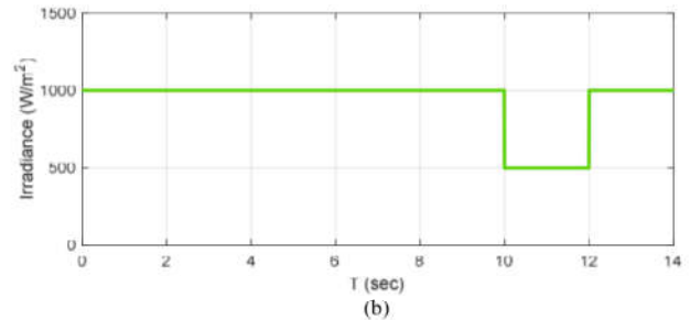
Fig. 5. Case studies. (a) Variable load profile, (b) Solar irradiance change
